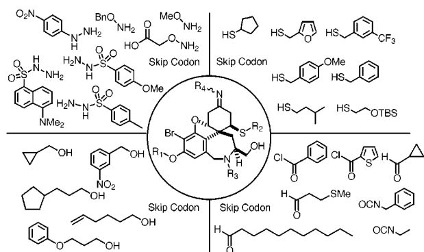
Figure 2. Building blocks used in the library synthesis.
