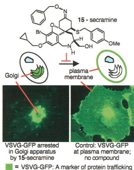
Figure 3. Discovery of secramine , a galanthamine-based molecule that perturbs protein trafficking.
