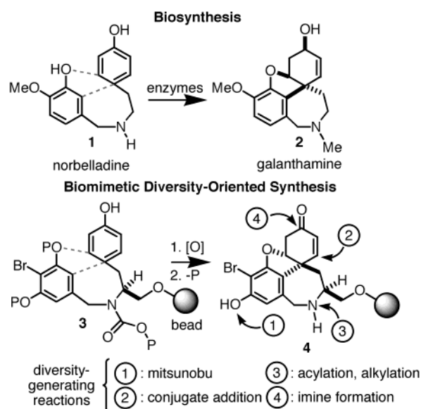
Figure 1. Biomimetic diversity-oriented synthesis parallels the biosynthesis of galanthamine.
